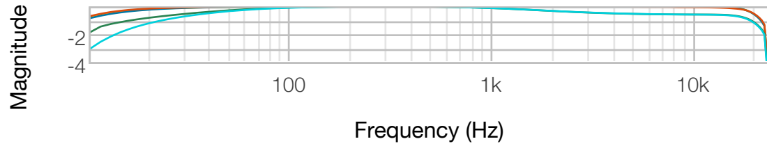
Frequency Response (1/24 Octave Smoothing)
