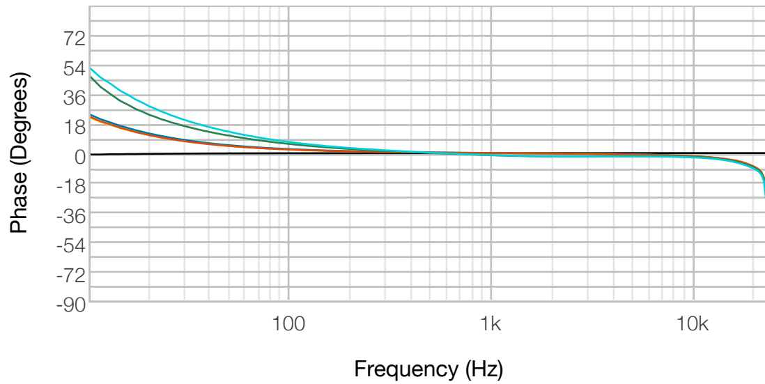
Minimum Phase Response (1/24 Octave Smoothing)
